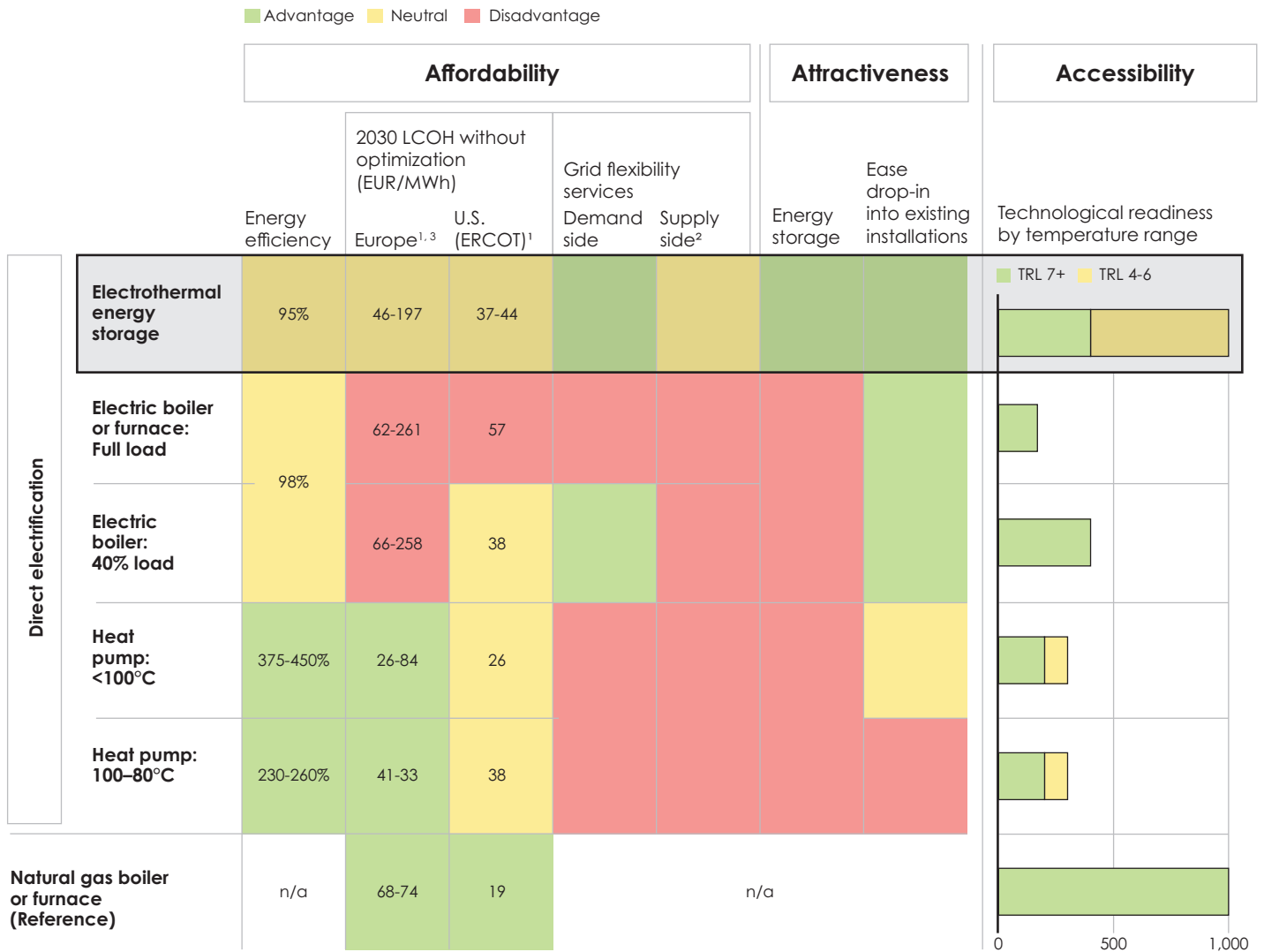
Figure 8 Key differences between ETES, heat pump and e-boiler technologies
