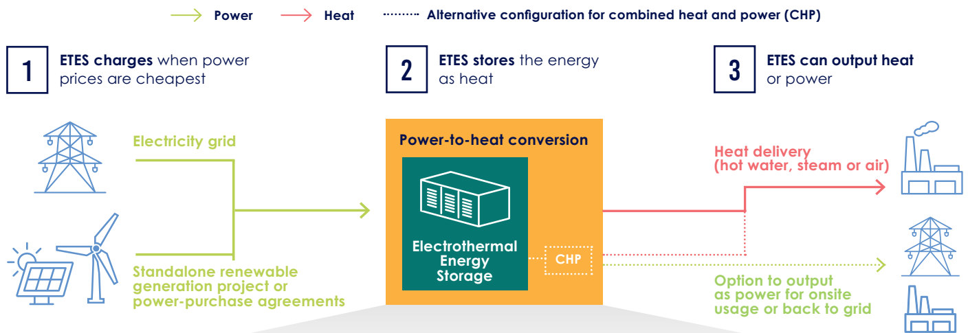
Figure ES1 How different types of ETES technologies work
